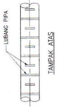
PIPA LINDI LUBANG MELINTANG NTS
