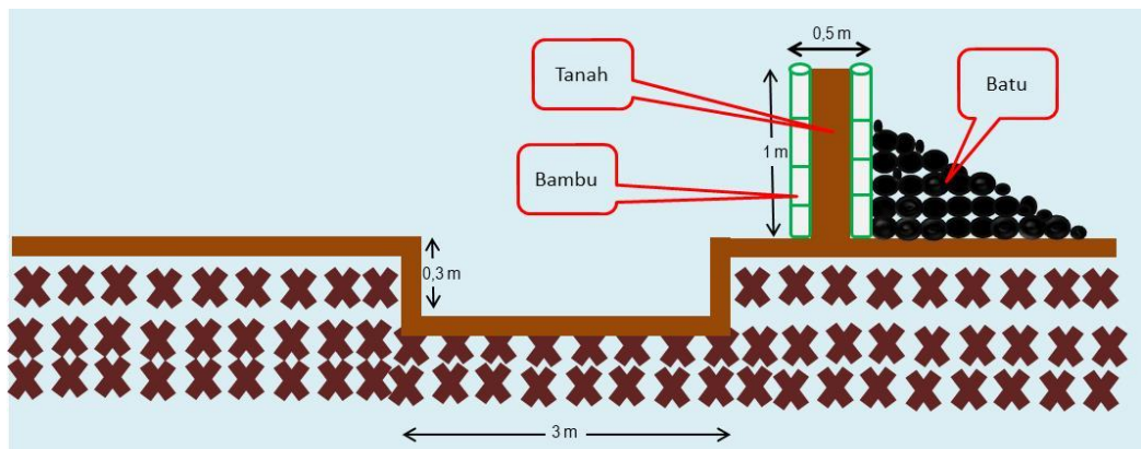
Gambar 4.47. Ilustrasi bio gully plug tampak samping
