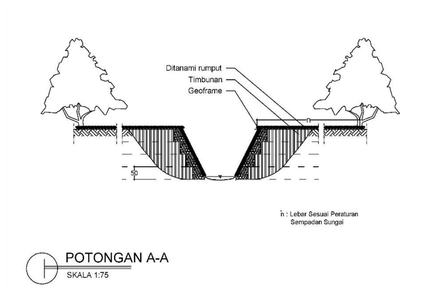
Gambar 4.78. Geoframe Tampak Samping
