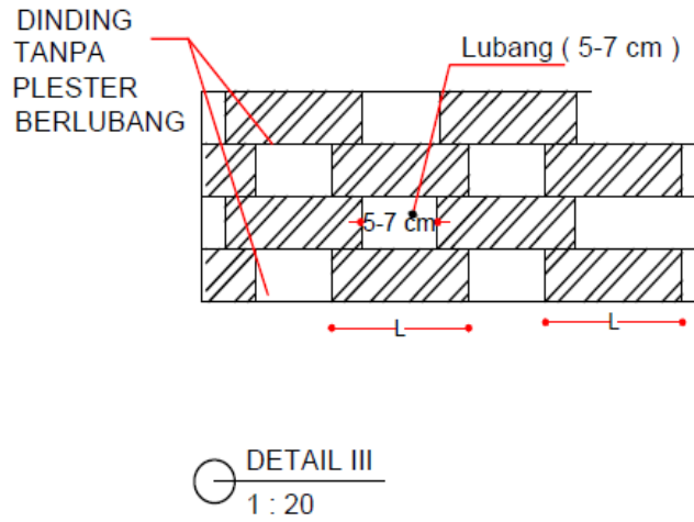
Gambar 4.62. Dinding SRA
