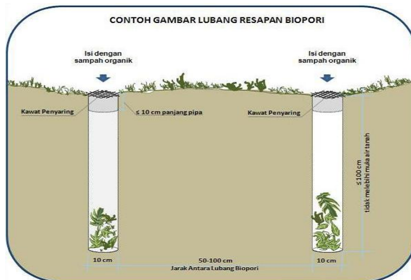
Gambar 4.93. Lubang Resapan Biopori (LRB)
