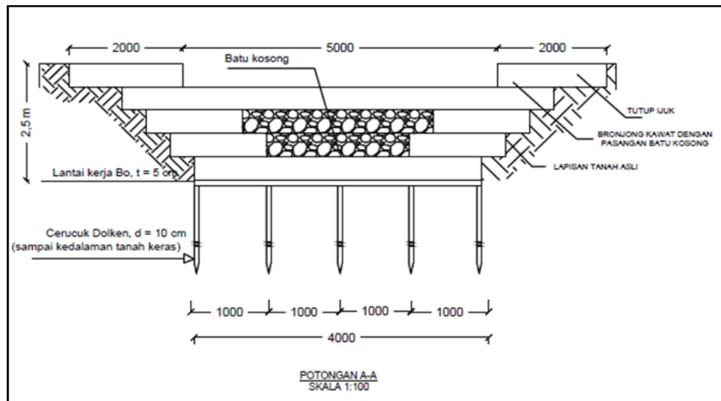
Gambar 4.16. Dam Penahan Batu Bronjong tampak samping
